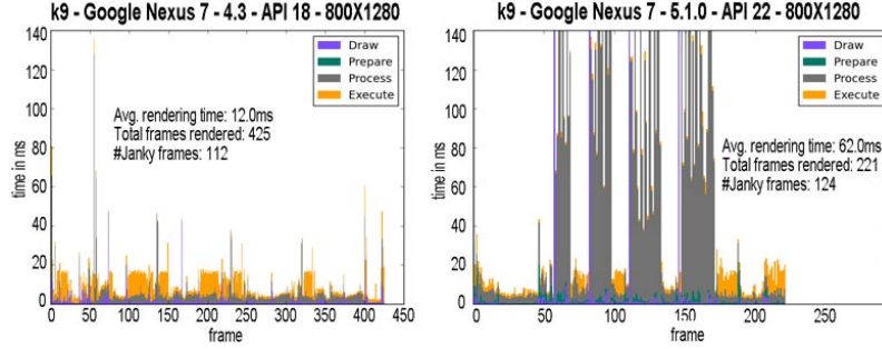
Figure 7: Frames rendered during the test scenario execution in the K-9 app in the historical dataset (left) and in the new context (right).
