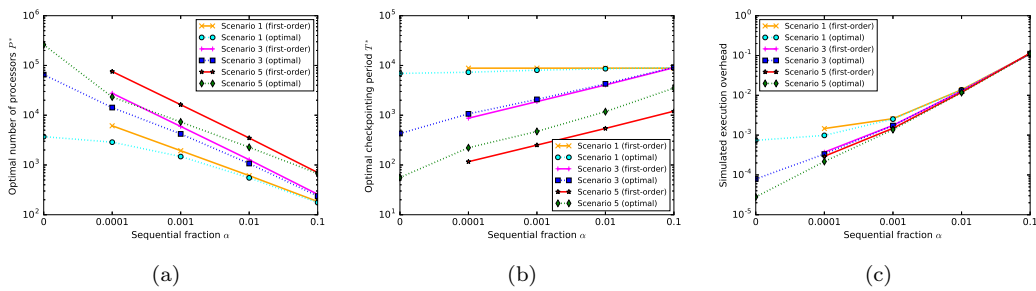
Figure 4: Optimal checkpointing period T^* and number of processors P^* (from Theorems 2 and 3, and from numerical solution), as well as the simulated execution overhead under different sequential fraction \alpha on platform Hera.
