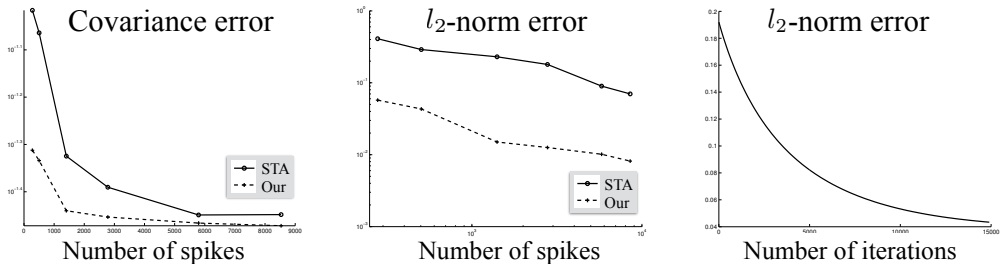
Figure 3: Convergence of the approach: (left) covariance error (1 - \frac{cov(u, u_0)}{\sigma_u \sigma_{u_0}}) as a function of the number of spikes in semi-log scale, (middle) l_2 -norm error (\|u - u_0\|_2) as a function of the number of spikes in log-log scale, and (right) l_2 -norm error as a function of the number of iterations for N_t = 1000 .
