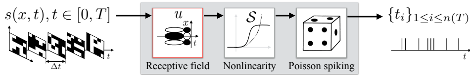
Figure 1: Illustration of the LNP model (1). Two kinds of \mathcal{S}(\cdot) are illustrated: ramp- or sigmoid-like nonlinearities. Here the stimulus is a white noise sequence which is the classical stimulus used for the spike-triggered averaged approach (STA, see [6]).
