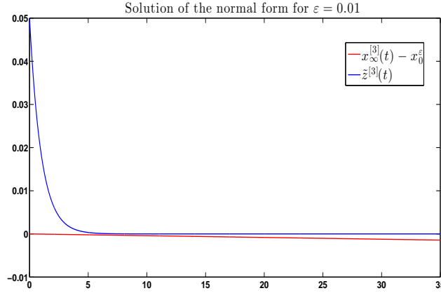
Figure 6: Solution (x_\infty^{[3]}(t), \tilde{z}^{[3]}(t)) of (3.3) for x_0 = 0.8 , z_0 = 0.05 and \varepsilon = 0.01 .
