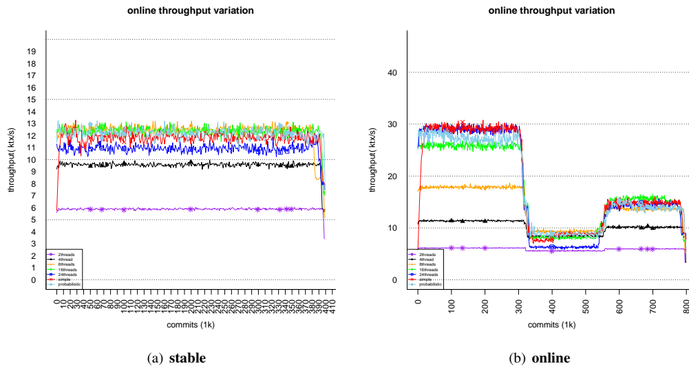
Figure 13: Online throughput variation of EigenBench . The red line with crosses and the sky blue line with circles is the simple model and probabilistic model respectively.
