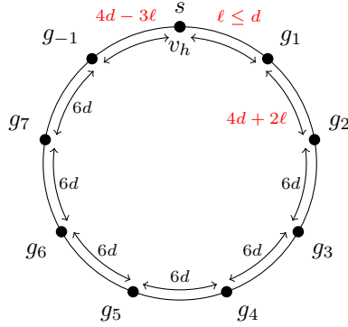
Figure 1: General position in the case k = 8, s = 2
