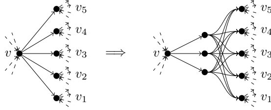
Figure 4: Constructing R_8(\mathcal{F}) from R_6(\mathcal{F})
