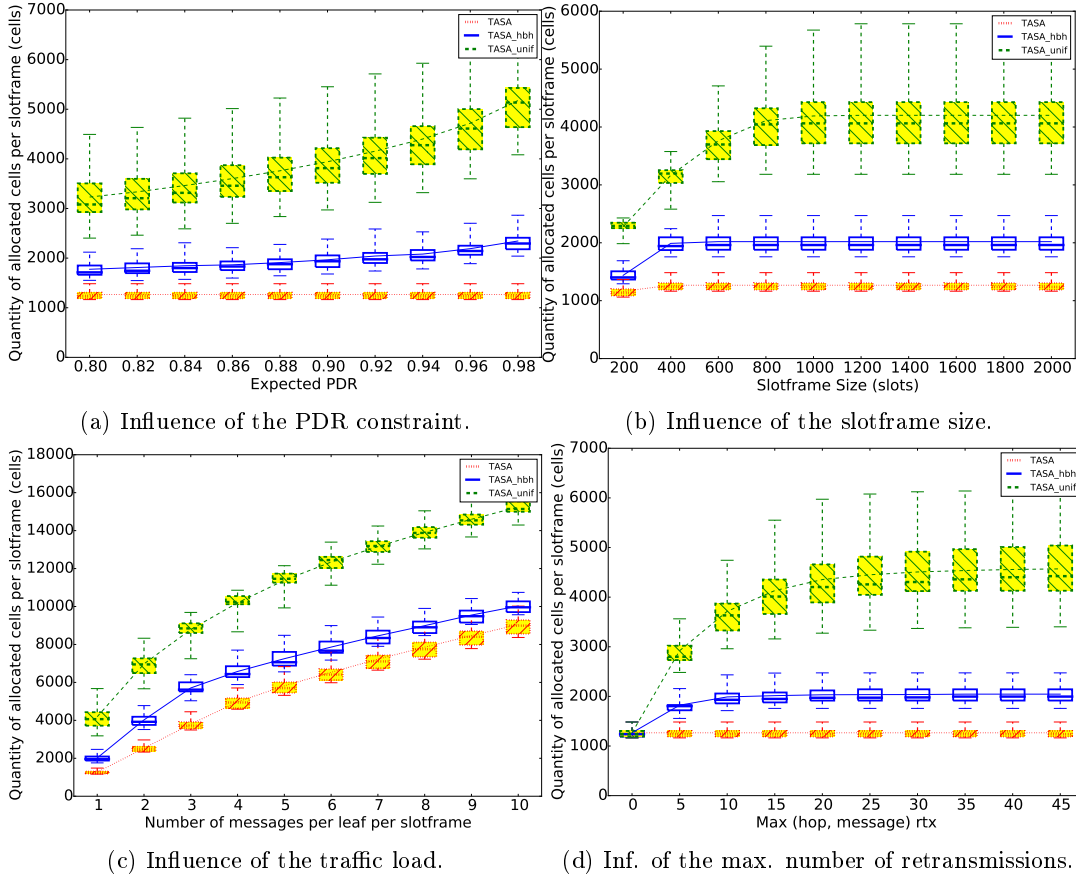
Figure 5: Evaluation of the performance in terms of network resource usage.
