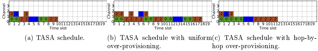
Figure 1: Example of FTDMA Schedule shapes built by TASA and by the proposed extensions. Based on a tree topology with 3 leaves, 3 relays, 1 gateway. Each leaf sends 1 message of a given application. The blue app. message is a single frame while the two other app. have messages of 2 fragments. The track IDs are shown in the cells.
