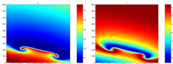
Spatial distribution of species at t = 400
