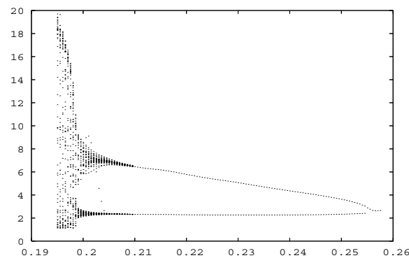
Figure 3. Bifurcation diagram when the parameter b varies.
