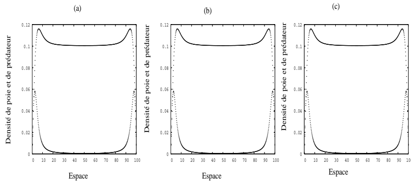
Figure 1. System (4) density of spatial distribution, the parameters and initial data are fixed as given in (31) and (32) and b = 0.256
