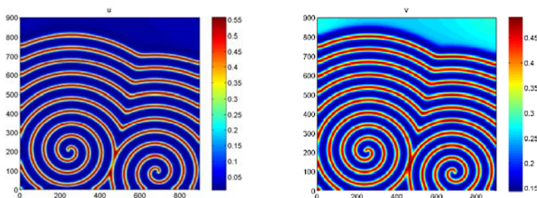
Figure 4. Spatial spiral waves type distribution of species at t = 1200 for respectively the prey and the predator. Initial conditions are given in (35). b = 0.042 , e_2 = 0.2 , the other Parameters are given in (36)
