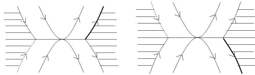
Figure 6. Funnel and anti-funnel : On the left the case a > 0 , on the right the case a < 0 .
