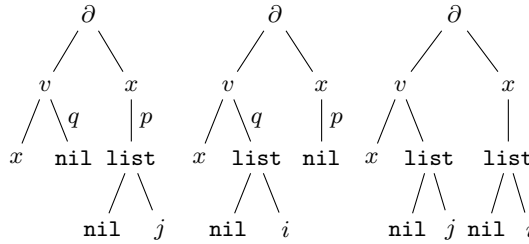
Fig. 3. The elementary CE-strategy (@q.\tau) \vee (@p.\tau') , that is the combination of the two elementary CE-strategies @q.\tau and @p.\tau' , and its application to the term t = \partial_x v(x) , yielding the term \partial_{x_j} v_i(x) .
