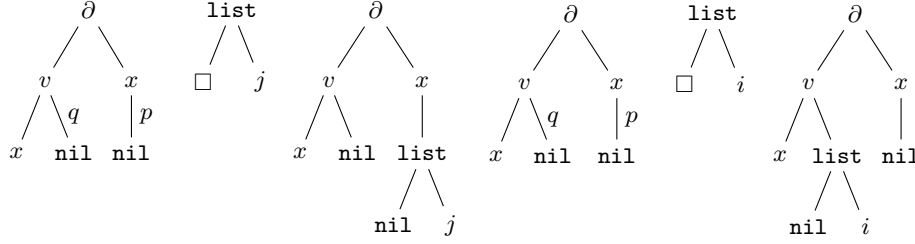
Fig. 1. Application of the elementary CE-strategy @p.\tau (with the context \tau = \text{list}(\square, j) ) to the term t = \partial_x v(x) at the position p , yielding the term \partial_{x_j} v(x) .
