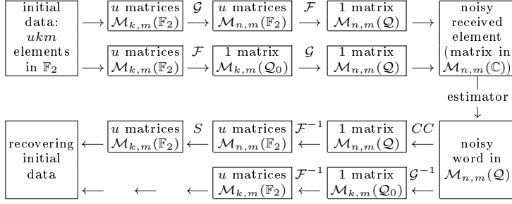
Figure 1 This figure represents the different coding and decoding schemes described in this section:
