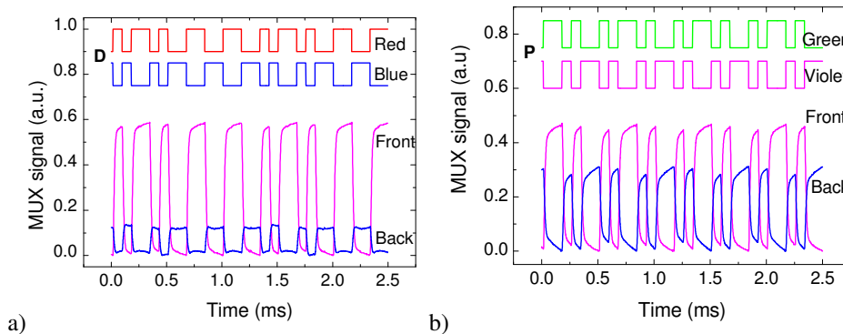
Fig. 9. Two digital light signals a) D [R, B] and b) P [G, V].
