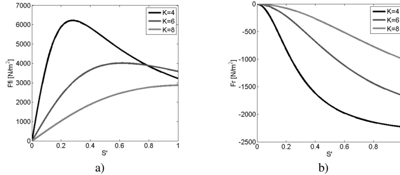
Fig. 8. Influence of the EMF's wavelength in the density force components on rotor: (a) tangential component; (b) radial component. S' = (\omega - k\omega_r)/\omega .
