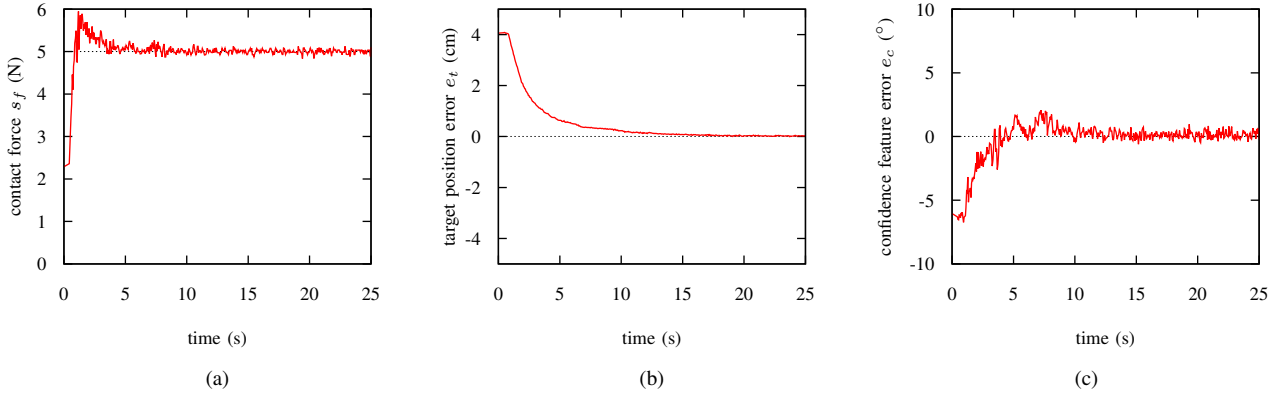
Fig. 5. Convergence: Evolution of the features during convergence in a static environment. (a) Contact force s_f in N. (b) Target position error e_t in cm. (c) Confidence feature error e_c in degrees.
