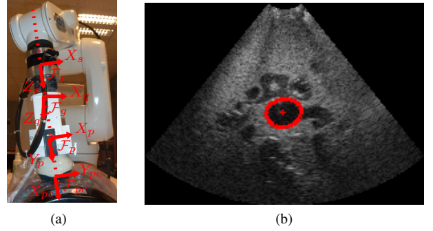
Fig. 1. (a) Robotic system and the corresponding force sensor frame ( \mathcal{F}_s ), probe frame ( \mathcal{F}_p ), probe contact frame ( \mathcal{F}_{pc} ), and gravity frame ( \mathcal{F}_g ). (b) An ultrasound image. The red line corresponds to the contour of the target. The red cross corresponds to the barycenter of the target.
