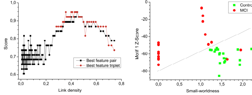
Fig. 3. (Left) Classification score as a function of link density; black (red) points indicate the best classification score obtained using pairs (triplets) of features. (Right) Classification of MCI and healthy subjects; green (red) points represent the position in the space of features of healthy (MCI) patients. Adapted from Ref. [20].
