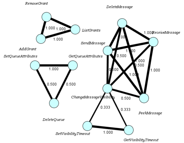
Fig. 6. G_{MessageQueue}^{dom} for MessageQueue.
