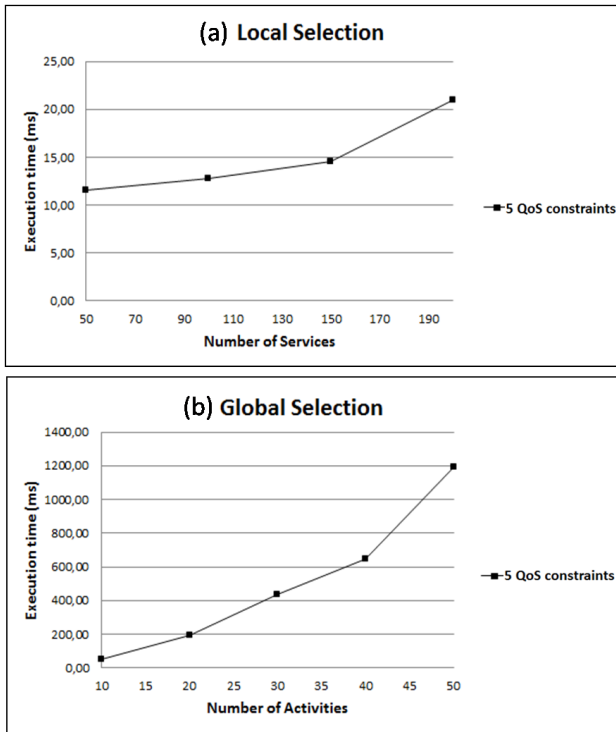
Fig. 4. Execution time of the (a) local selection and (b) global selection of our distributed QoS-aware service selection algorithm
