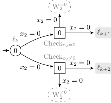
Fig. 10. Widget WZ_2 simulating zero-check for C_2
