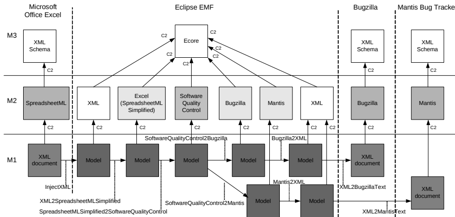
Figure 7 Excel-to-Bugzilla and Excel-to-Mantis bridges
