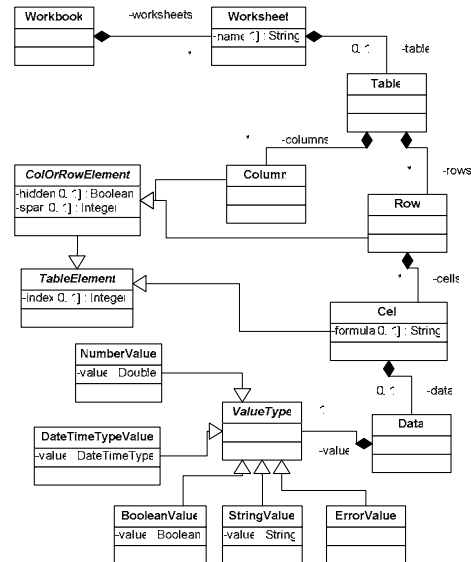
Figure 3 Simplified version of the Excel metamodel (SpreadsheetMLSimplified)
