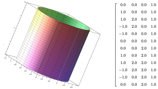
Figure 2: Degenerate case in inversion. A Bézier patch of degree (5, 1) with a seam edge and its control point matrix. The points on the seam have two pre-images. More cases shown in Figure 3.
