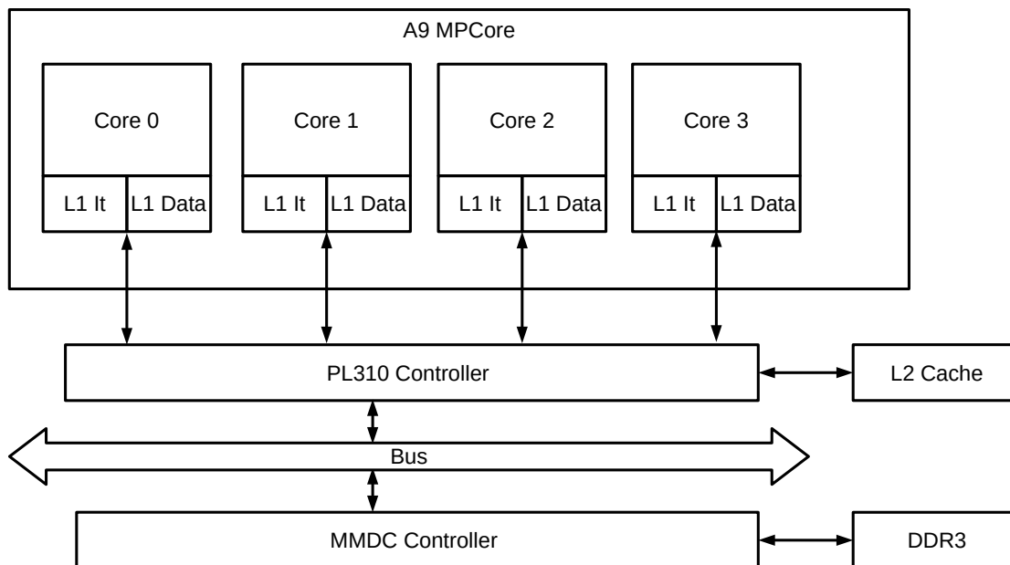
Figure 1: Architecture of the SABRE Lite board
