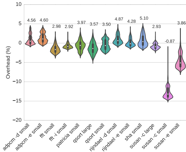
Figure 8: Overhead for MiBench applications with constant loads
