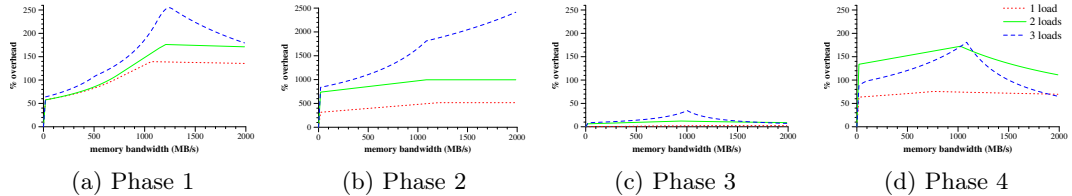
Figure 6: Overheads associated with the four phases of Susan small -c. Phase 2 has estimated overheads 10 times greater than the other phases.
