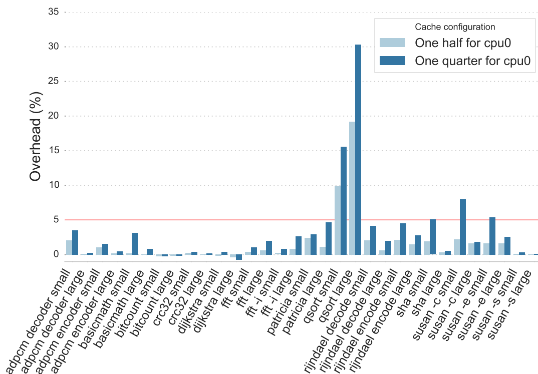
Figure 2: Impact of partitioning of MiBench performance
