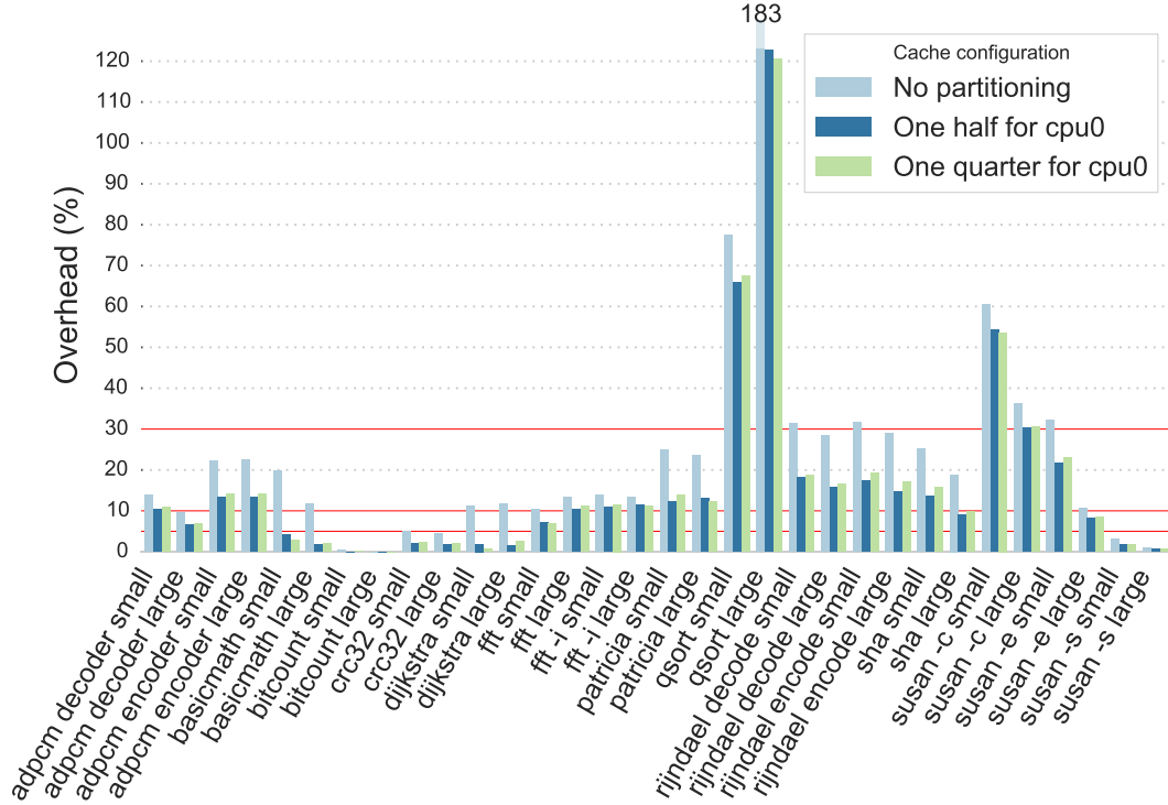
Figure 3: Impact of load on MiBench performance depending on the partitioning scheme
