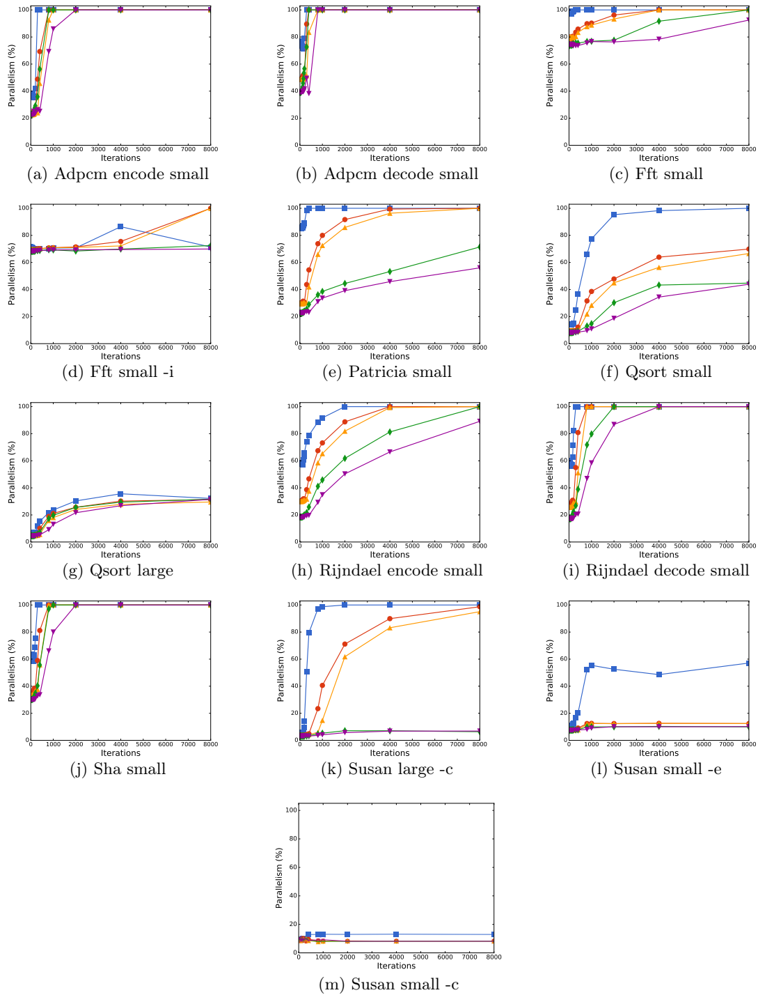
Figure 9: Parallelism for MiBench applications with constant loads
