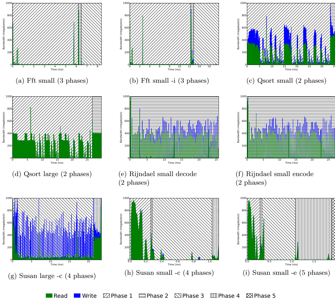
Figure 7: Memory profiles of selected MiBench applications
