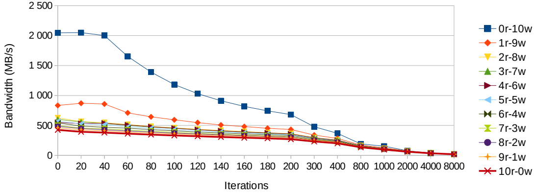
Figure 5: Bandwidth of the microbenchmark run in isolation
