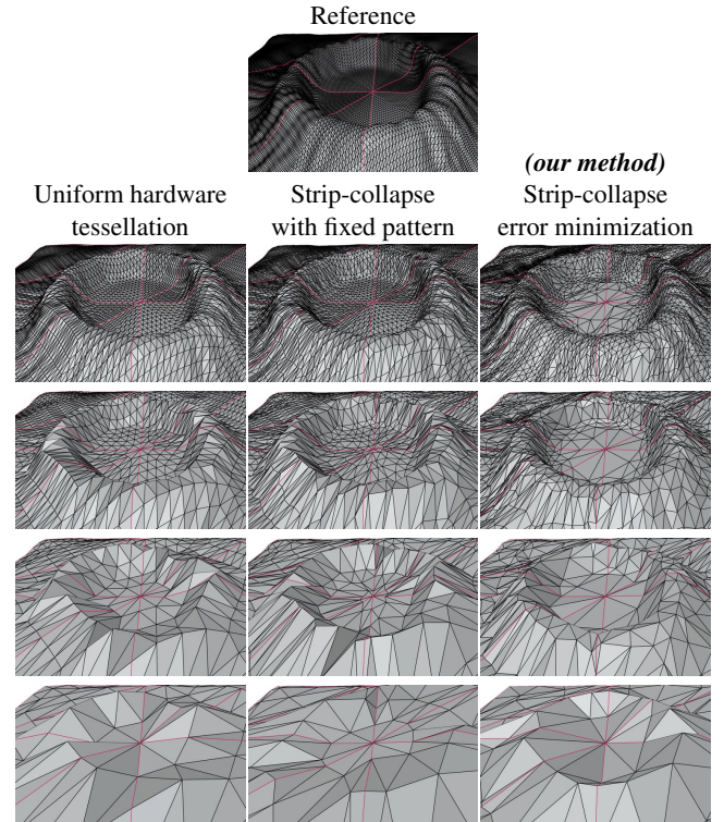
Figure 7: Starting from the same 8 patches and displacement map, comparison of the LOD representation generated by three approaches for the factors 32, 16, 8 and 4 (from top to bottom). Left: Uniform hardware tessellation. Middle: Mesh decimation constrained to choose the same strips as the tessellation pattern. Right: Our method, i.e., mesh decimation collapsing the strips that minimize an error metric. For each level, our approach better preserves the input geometry by spatially redistributing the polygonal size and density.
