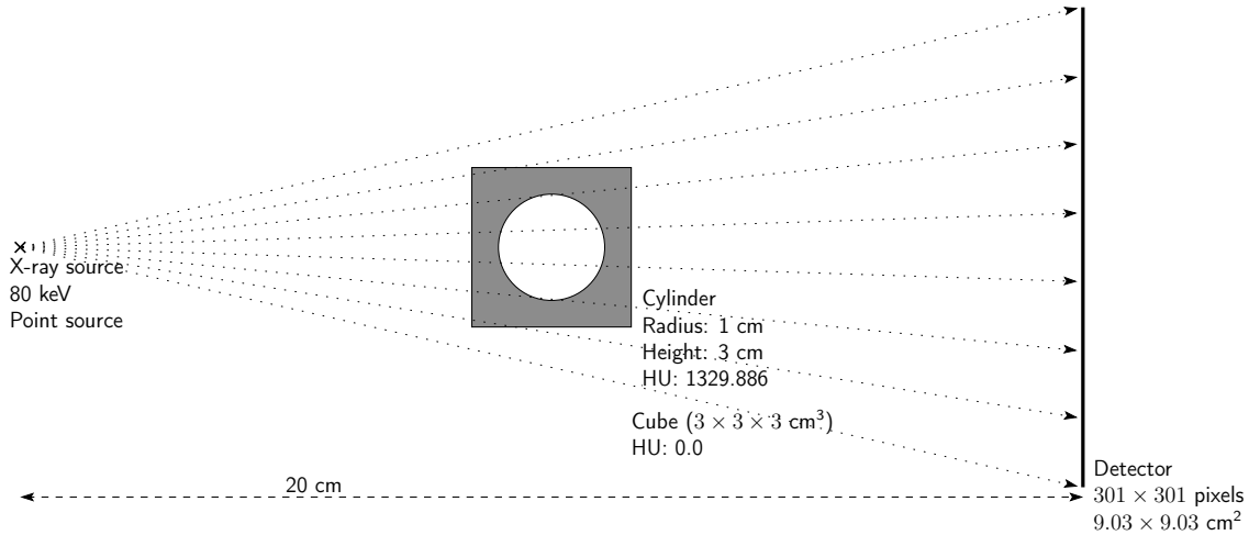
Figure 13: Simulation setup.
