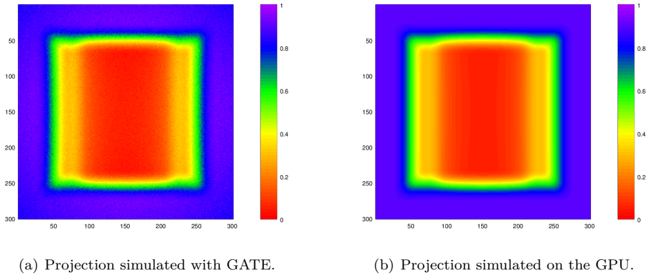
Figure 16: Projection using a cubic source.
