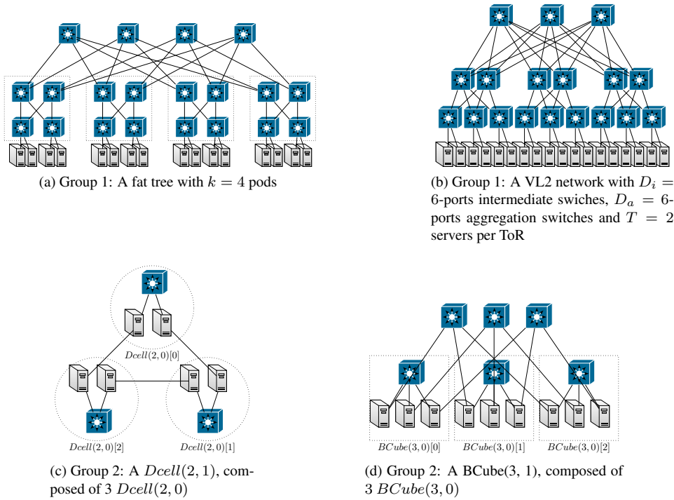
Figure 1: Example of topologies studied.
