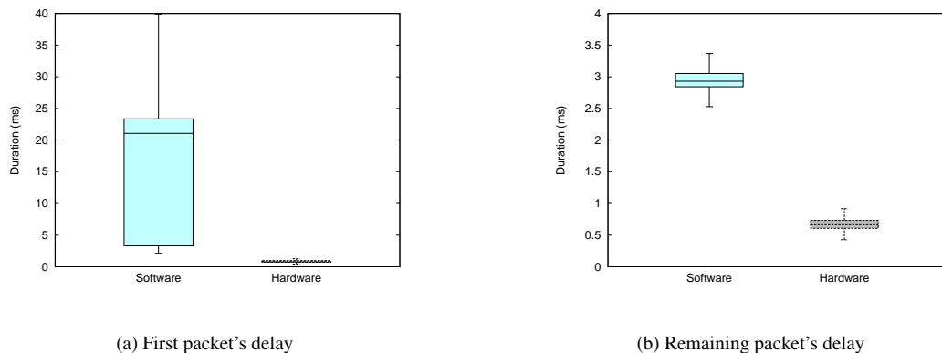
Figure 19: Packet delay boxplot
