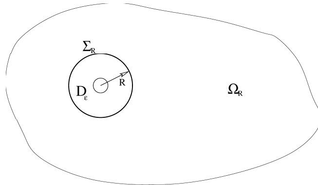
Figure 1. Domain truncation.
