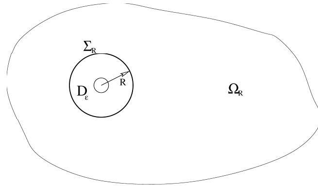
Figure 1. Domain truncation.
