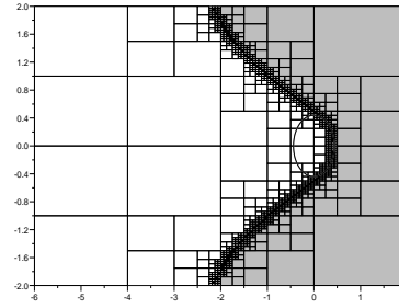
(b) L_{\max}=7 , T = 7.18 , # cells=952
