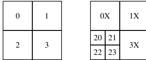
Figure 1. Refinement of a cell by quadrees
