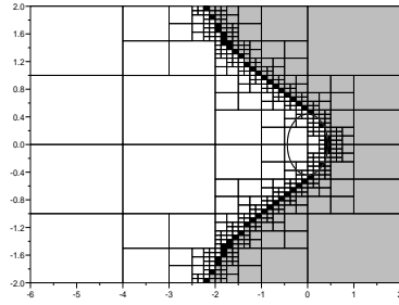
(a) L_{\max}=6 , T = 12.96 , # cells=478
