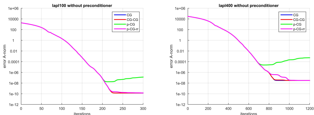
Figure 1: Error history for the different CG methods applied to the 1ap1100 (left) and 1ap1400 (right) matrices, see Table 1. Error A-norm \|\hat{x} - x_i\|_A in function of iterations for CG (blue), Chronopoulos/Gear CG (red), pipelined CG (green) and p-CG-rr (magenta).
