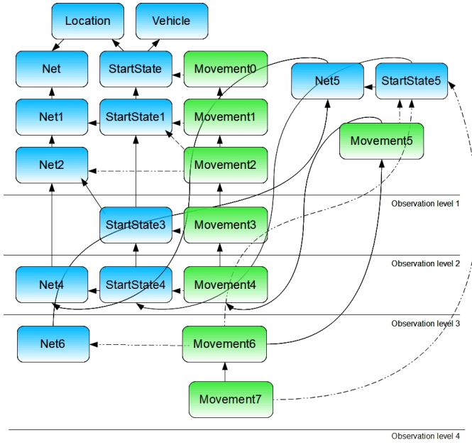
Fig. 5. Event-B model of the land transport domain [25]
