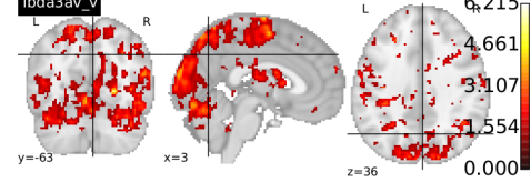
(b) Multivariate Hurst exponent estimation ( \lambda = 3 ).
