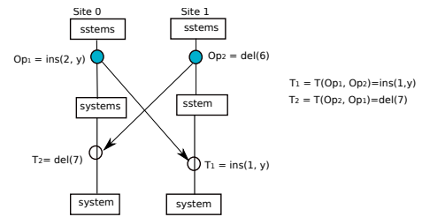
Figure 2. Integrate operation in OT algorithms
