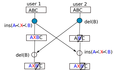
Figure 5. Integration in WOOT
