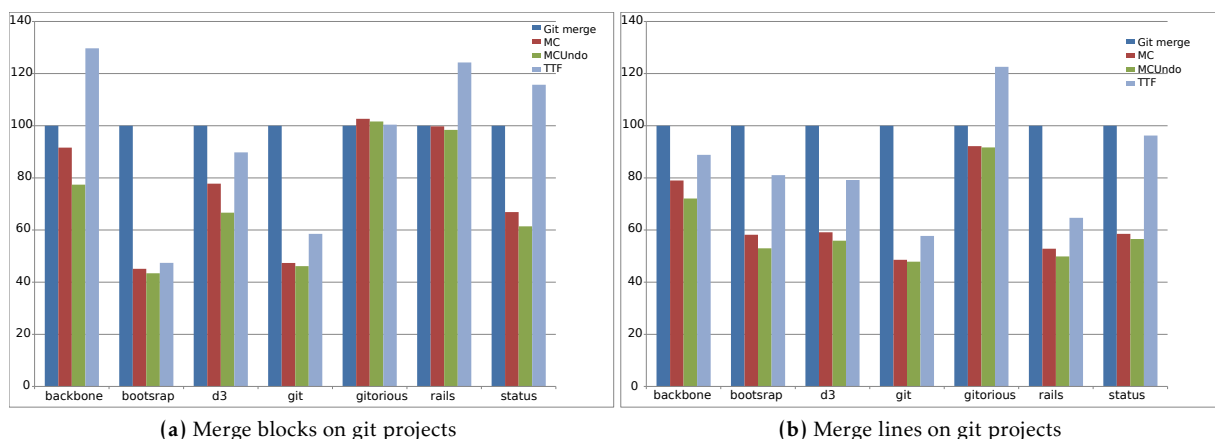
Figure 13. Merge blocks and merge lines
