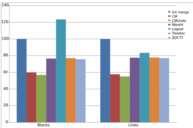
Figure 14. Total merge block and merge line
