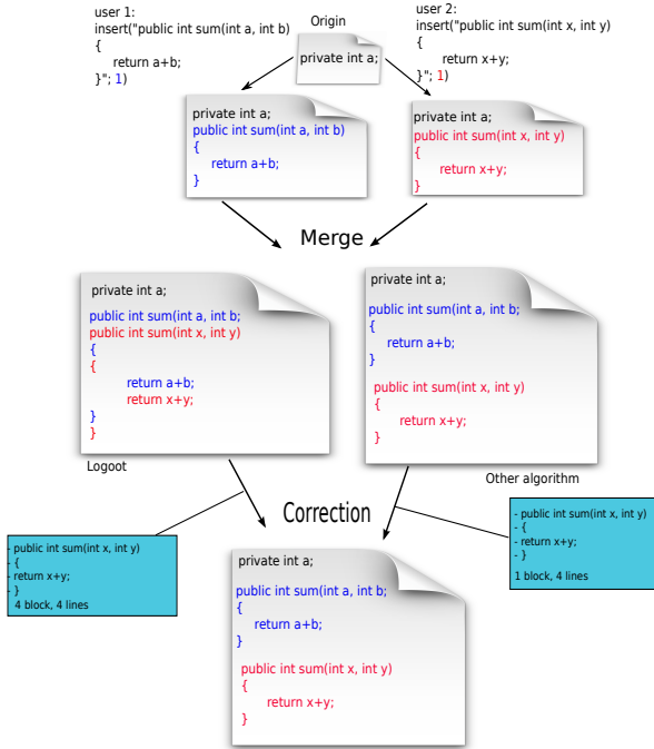
Figure 7. Different merge in operation-based approaches
