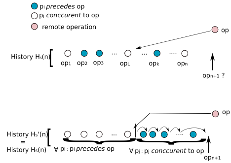
Figure 4. Integrate a remote operation in SOCT2
