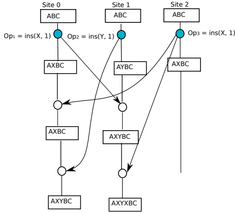
Figure 12. ACM divergence by using traditional OT
