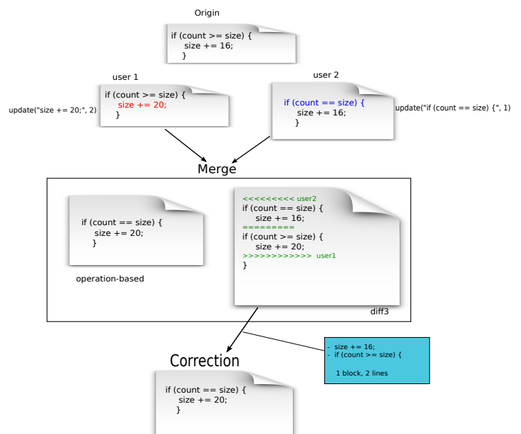
Figure 9. Concurrent consecutive modifications
