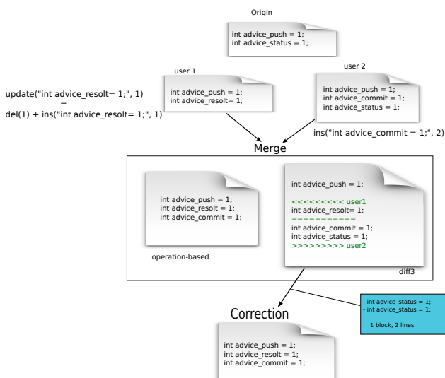
Figure 8. Addition at the same position
