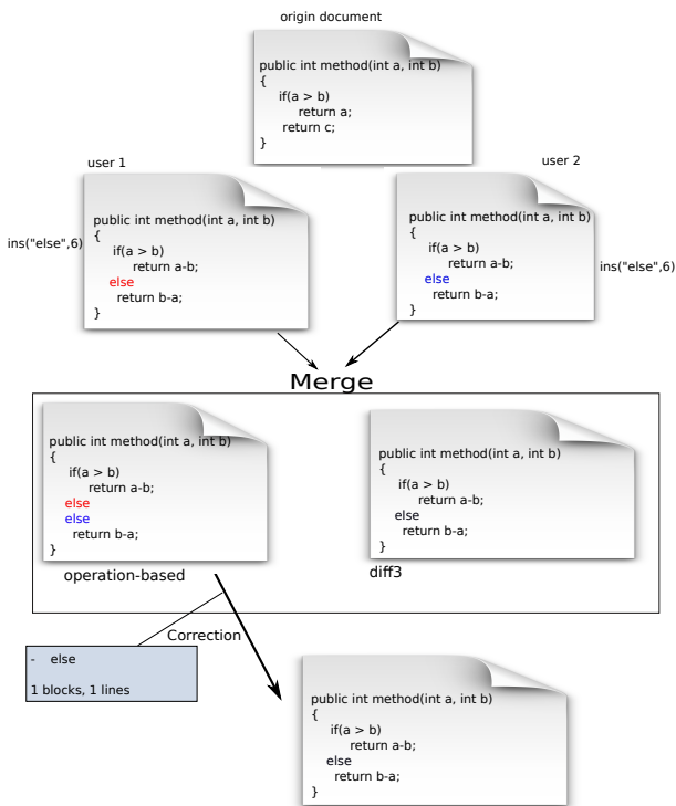
Figure 10. Accidental clean merge
