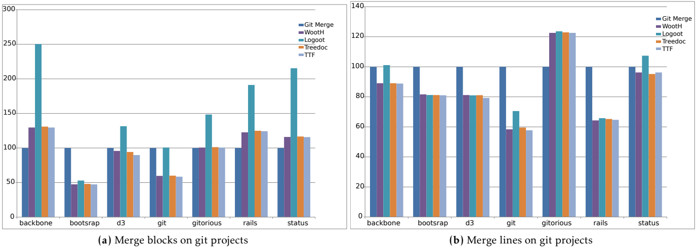
Figure 6. Merge blocks and merge lines
