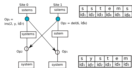
Figure 3. Integrate operation in CRDT algorithms
