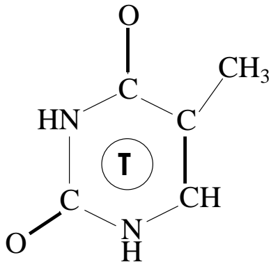
Thymine
