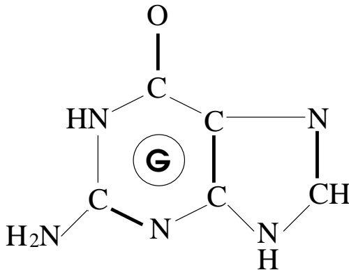
Guanine
