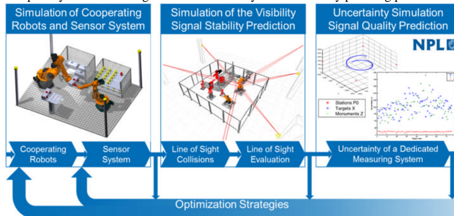
Figure 5: Metrology infrastructure for multi robotic cooperative assembly
