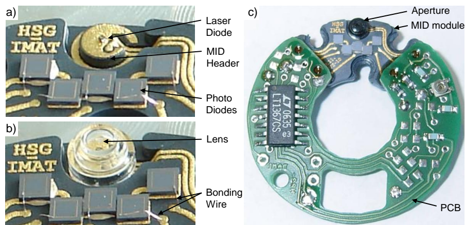
Fig. 1. a) MID-substrate with assembled laser diode and photo diodes; b) MID-substrate with assembled lens; c) MID module inclusive the assembled aperture connected to the PCB
