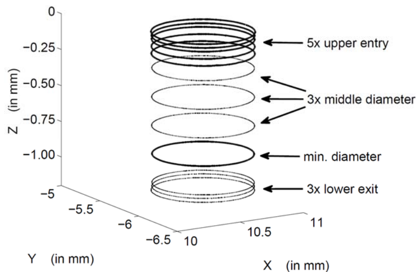
Fig. 2. Typical example of a hole diameter measurement by micro-CMM. The results showed that drilled-bored holes are not cylindrical as usually modeled and that a tightening of 1\text{--}4 \text{ } \mu\text{m} exists at 50\text{--}100 \text{ } \mu\text{m} above the lower hole exit. Measure parameters. 52 runs, probe diameter 302 \text{ } \mu\text{m} , nominal hole diameter 990 \text{ } \mu\text{m}
