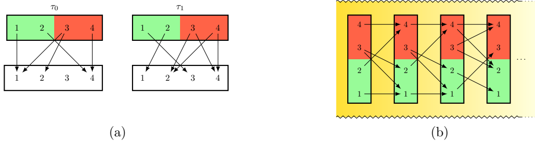
■ Figure 1 (a) Semi-tiles \tau_0 and \tau_1 such that (\tau_0, \tau_1) represents the tile \{(1, 1, 3), (2, 4, 1), (3, 1, 2), (3, 2, 4), (4, 4, 2), (4, 4, 4)\} with Q_{\exists} = \{1, 2\} and Q_{\forall} = \{3, 4\} . (b) Representation of the sequence of semi-tiles \tau_0 \tau_0 \tau_1 \dots
