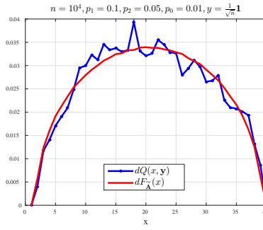
Fig. 2. Asymptotic spectral function for symmetric SBM, \mathbf{y} = 1/\sqrt{n}\mathbf{1} .
