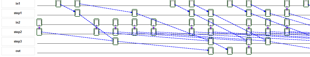
Figure 9: A valid schedule for the application part of Fig. 8
