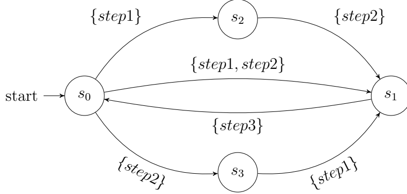
Figure 11: Synchronized product of Eqs. 1-3 and Eq. 5.
