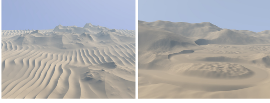
Figure 17: Examples of terrains rendered in real-time using the accelerated sphere tracing algorithm. Using sphere tracing instead of adaptive tessellation allows us to render faster and without visual artifacts detailed and sharp geometries such as those sand dunes.
