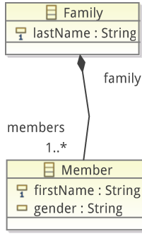
Fig. 1 Families metamodel
