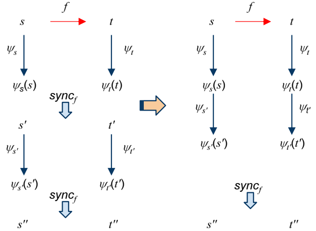
Fig. 13 Composability Feature
