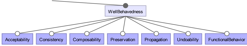
Fig. 11 Well-behavedness properties
