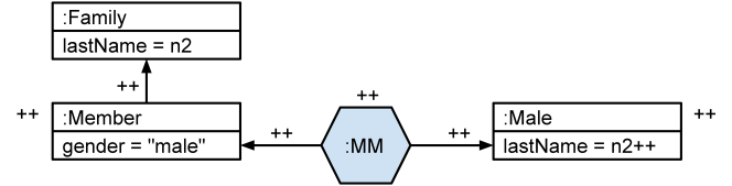
Member2Male()
