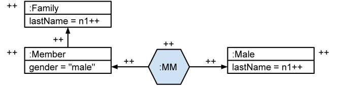
Member2Male()
