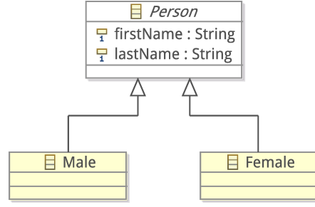
Fig. 2 Persons metamodel
