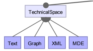
Fig. 5 Technical Space
