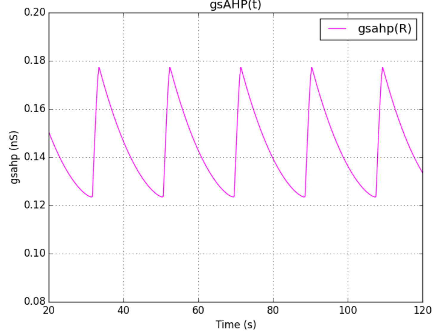
Figure C Simulated g_{sAHP}(t)
