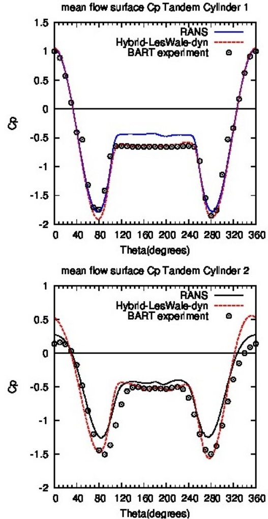
Figure 11. Tandem of cylinders: Mean pressure coefficient distribution and mean C_d .
