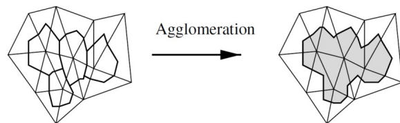
Figure 2. Building the VMS coarse level
