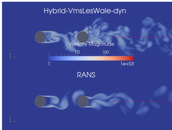
Figure 6. Tandem of cylinders: Vorticity magnitude - Hybrid VMS versus RANS.
