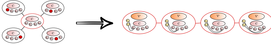
Figure 5: The 1-good path decomposition (right) obtained from the central bag with degree four (left).
