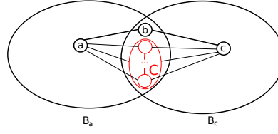
Figure 23: Case T_a \cap T_c = \emptyset .
