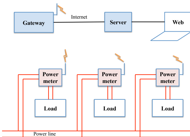
Fig. 1: Smart meter grid to observe and analyze the power consumption characteristic of electric devices.
