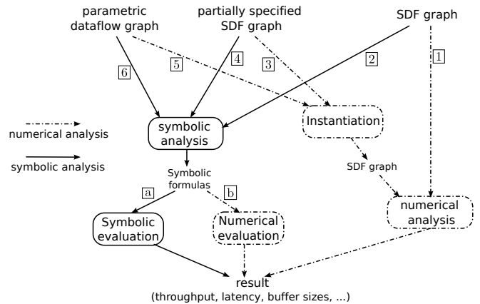
Fig. 1: Symbolic and numerical analyses.
