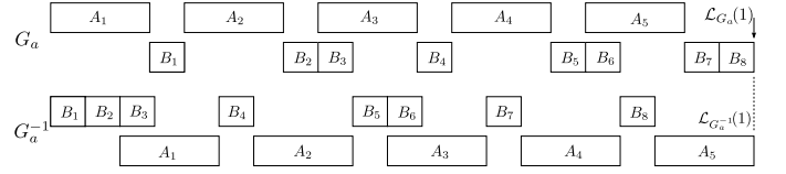
Fig. 4: Illustration of the duality theorem.
