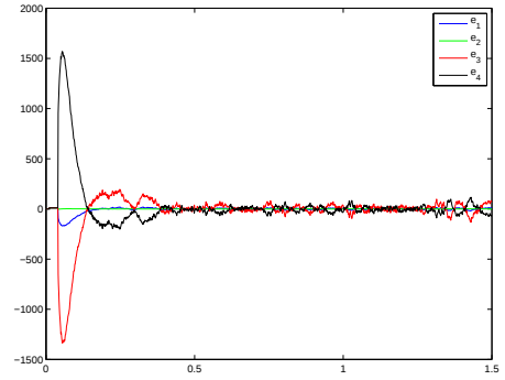
Figure 4: The observation error for h = 0.01 s with noisy measurement.
