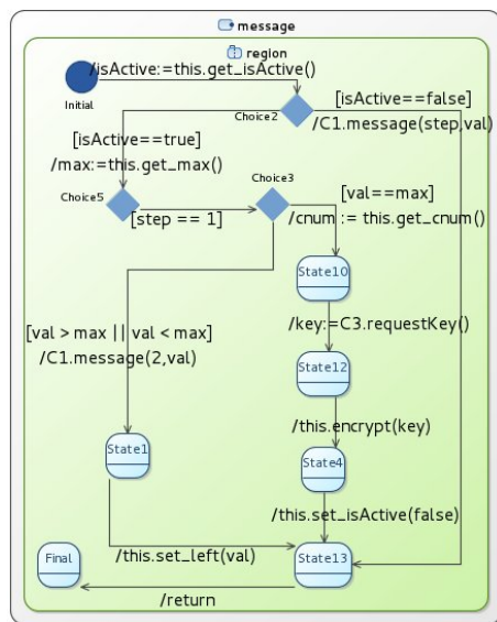
Figure 9: State Machine of the 1st phase of election algorithm
