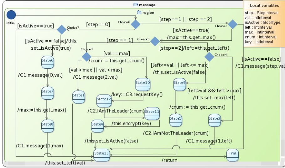
Figure 3: Message State Machine
