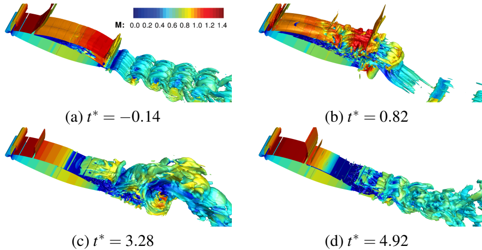
Figure 15: Instantaneous Q-criterion isosurfaces for Q(c/U)^2 = 75
