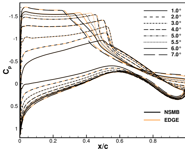
Figure 3: Comparison of the wall pressure coefficient between NSMB and Edge codes, for angles of attack between 1.0^\circ and 7.0^\circ
