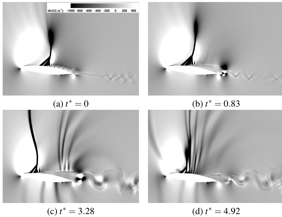
Figure 17: Divergence of velocity field - OES- k - \epsilon
