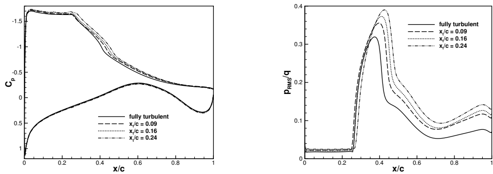
(a) Mean pressure coefficient (b) RMS value of pressure on the upper surface
