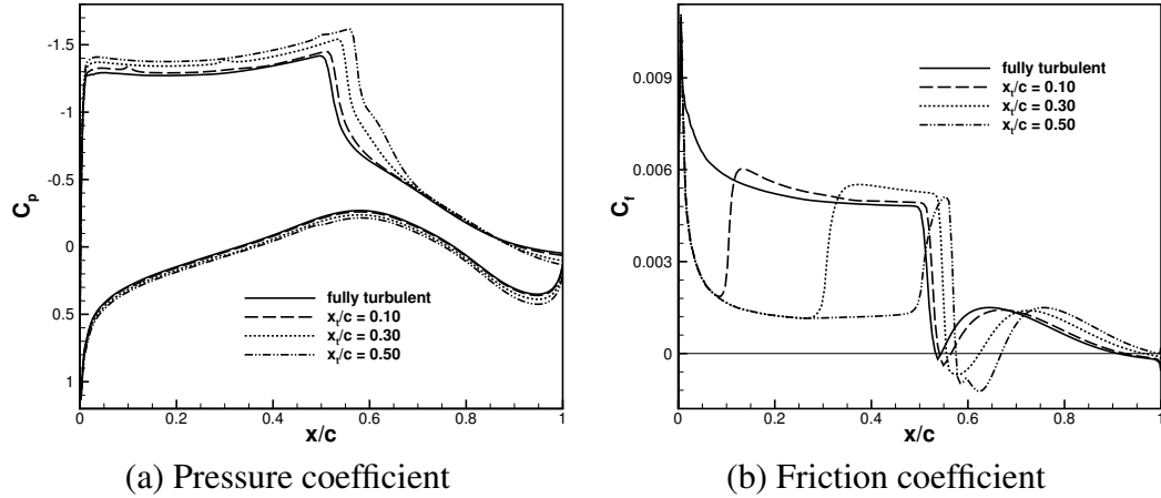
Figure 4: Steady surface distributions for selected transition locations
