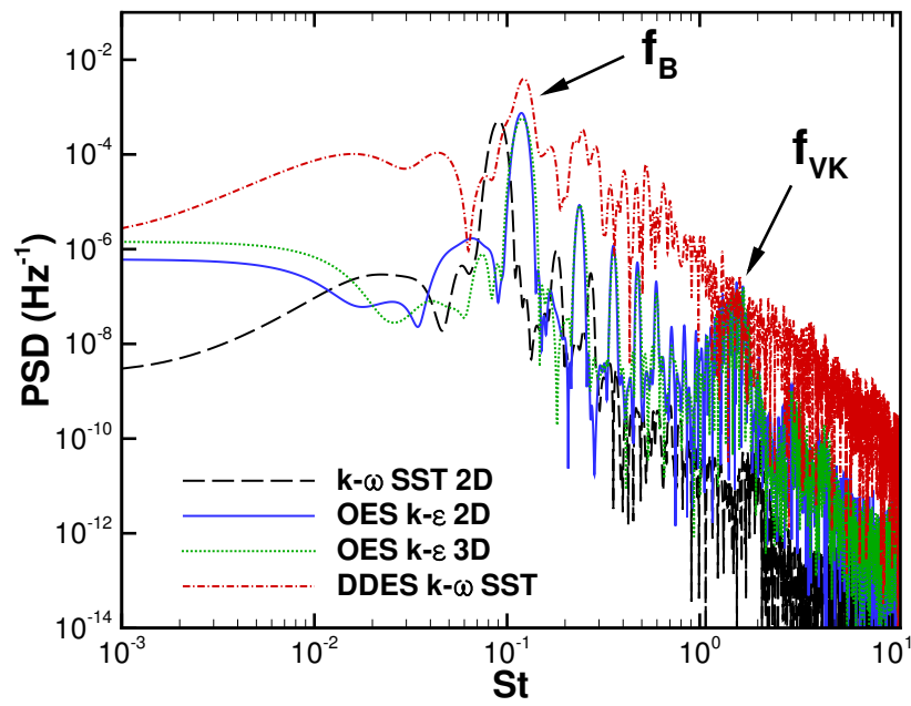
Figure 11: Comparison of the power spectra density of the lift coefficients time-dependent evolution between URANS k - \omega SST, 2D and 3D OES- k - \epsilon and DDES- k - \omega SST
