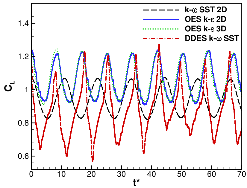
Figure 10: Comparison of the time-dependent evolution of the lift coefficients between URANS k-\omega SST, 2D and 3D OES- k-\epsilon and DDES- k-\omega SST
